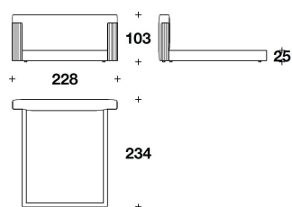
1CO (LE1) LETTO PER MATERASSO / BED FOR MATTRESS 165x200 - 228x234x103H. - H.B.25cm 65x78 2/3 - 89 2/3x92x40 2/3H. - H.B.9 3/4"
