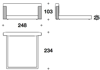
1CO (LE2) LETTO PER MATERASSO / BED FOR MATTRESS 185x200 - 248x234x103H. - H.B.25cm 73x78 2/3 - 97 2/3x92x40 2/3H. - H.B.9 3/4"
