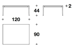
VTC (16) - VTC (16C) COFFEE TABLE 120x90x44H.cm 47 1/3x35 1/3x17 1/4H."
