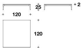
VTC (11) - VTC (11C) LOW : COFFEE TABLE 120x120x25H.cm 47 1/3x47 1/3x9 3/4H."
